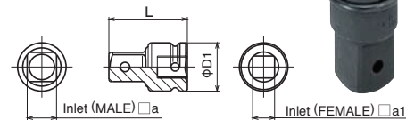
ADAPTER
