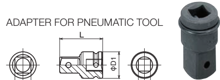
ADAPTER
